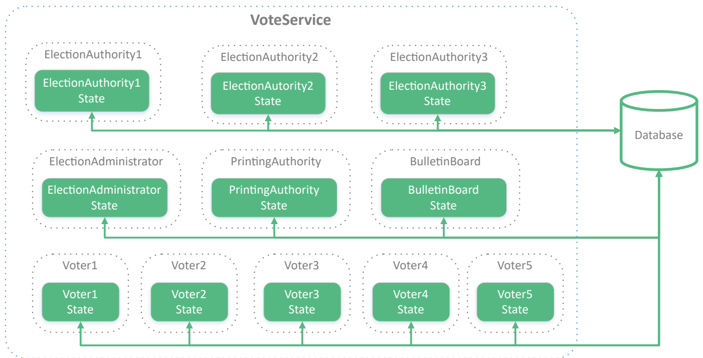
Figure 5.3: The internals of the VoteService: the functionality is divided into actor and state classes. The actors provide the functionality as described in the specification and by utilizing the crypto-library. The state is contained within the state classes that allow easy serialization both for persisting them to the database as well as to a JSON representation for the data synchronization.
